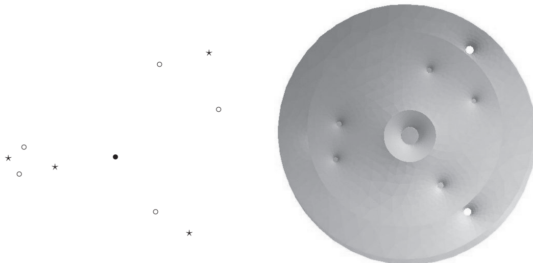
FIGURE 7. A genus-7 embedded asymmetric minimal surface (top view), computed from a configuration of type 4, 5, 1. The neck sizes are c_1 = \frac{3}{2} , c_2 = 1 , and c_3 = \frac{17}{5} .
