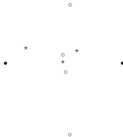
FIGURE 4. An asymmetric configuration of type 3, 4, 2 (embedded, genus 6). The neck sizes are c_1 = \frac{7}{10} , c_2 = 1 , and c_3 \approx 2.85 .
