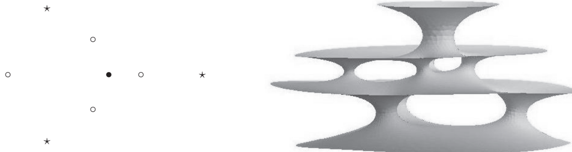
FIGURE 1. A configuration of type 3,4,1 and a genus-5 embedded minimal surface in the corresponding family. The stars, the circles, and the dot represent the points at levels 1, 2, and 3, respectively. The neck sizes are c_1 = \frac{7}{4} , c_2 = 1 , and c_3 \approx 2.34 .
