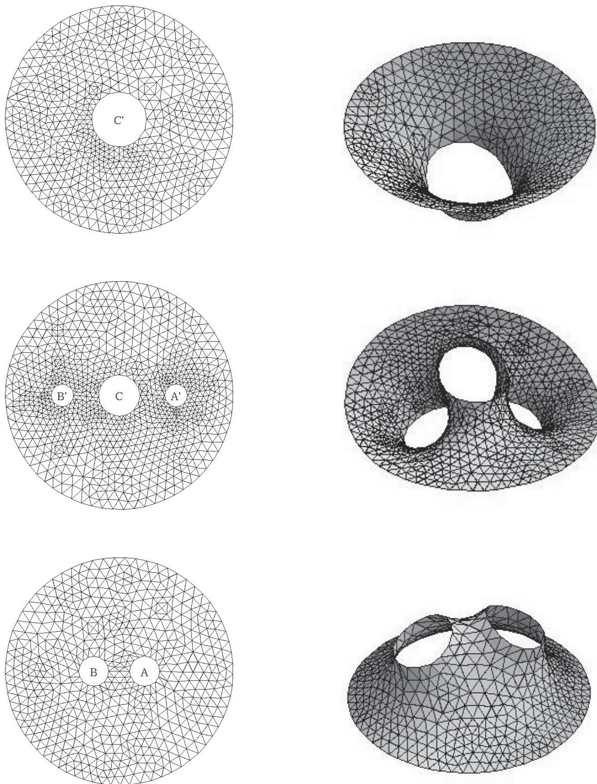
FIGURE 6. Triangulation of the three multicircular domains generated with MATLAB (left) and their image in space (right), in the case of the Costa–Hoffman–Meeks genus-1 surface. The three pieces on the right match perfectly, to give the whole surface.
