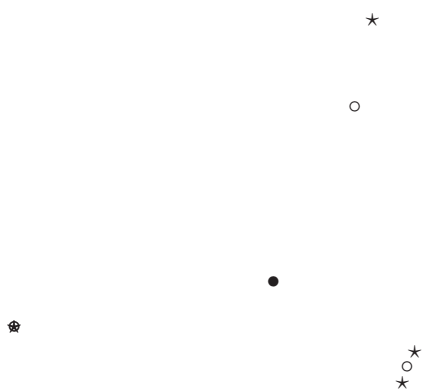
FIGURE 5. An asymmetric configuration of type 5, 4, 1. The neck sizes are c_1 = 1 , c_2 = 1.01 , and c_3 \approx 2.98 . There is a cluster of four points on the left and a cluster of three points on the right. This configuration is almost singular.
