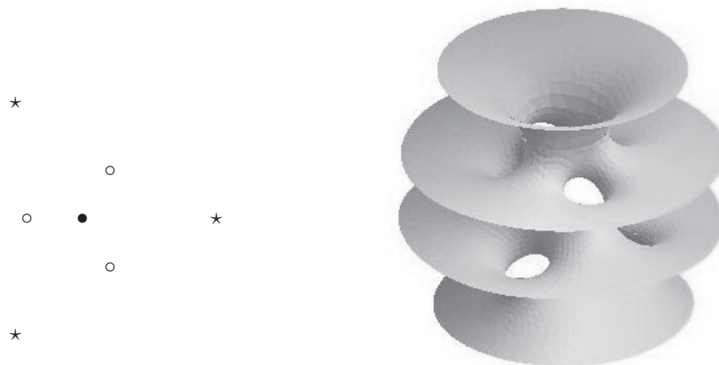
FIGURE 3. A configuration of type 3,3,1 with dihedral symmetry and a genus-4 embedded minimal surface in the corresponding family. The neck sizes are c_1 = 1.35 , c_2 = 1 , and c_3 = 1.595 .
