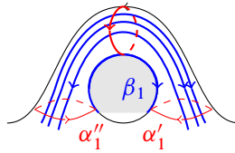
Figure 20: How the \beta_j look near the handles' cores
