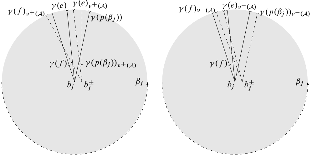
Figure 11: The orthogonal projections of \gamma(d)_\parallel on \mathcal{B}_j near b_j (where \sigma(p(\beta_j)) = \sigma(f) = 1 = -\sigma(e) )
