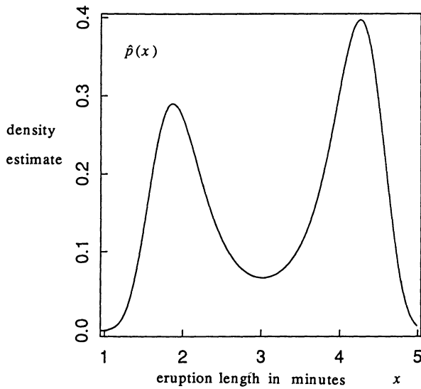
FIG. 1. Exponential family estimate for Old Faithful Geyser data using a polynomial of degree 4.
