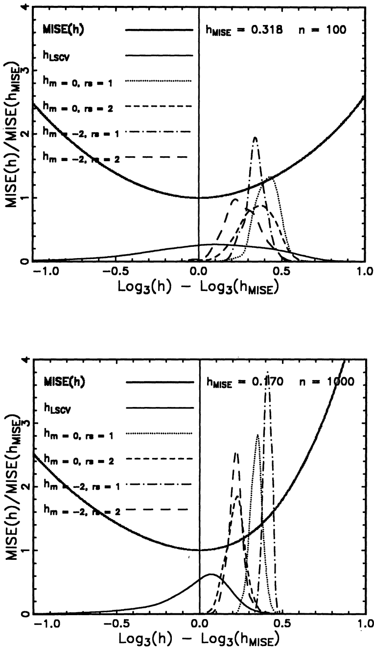
FIG. 1. MISE(h) together with kernel estimates of densities of selected bandwidths, for (a) n = 100 , (b) n = 1000 , for an asymmetric bimodal mixture density. In all cases \Delta = 1 . The symbol r_s gives reference step, that is, step number where N(0, \hat{\sigma}^2) reference distribution is used.
