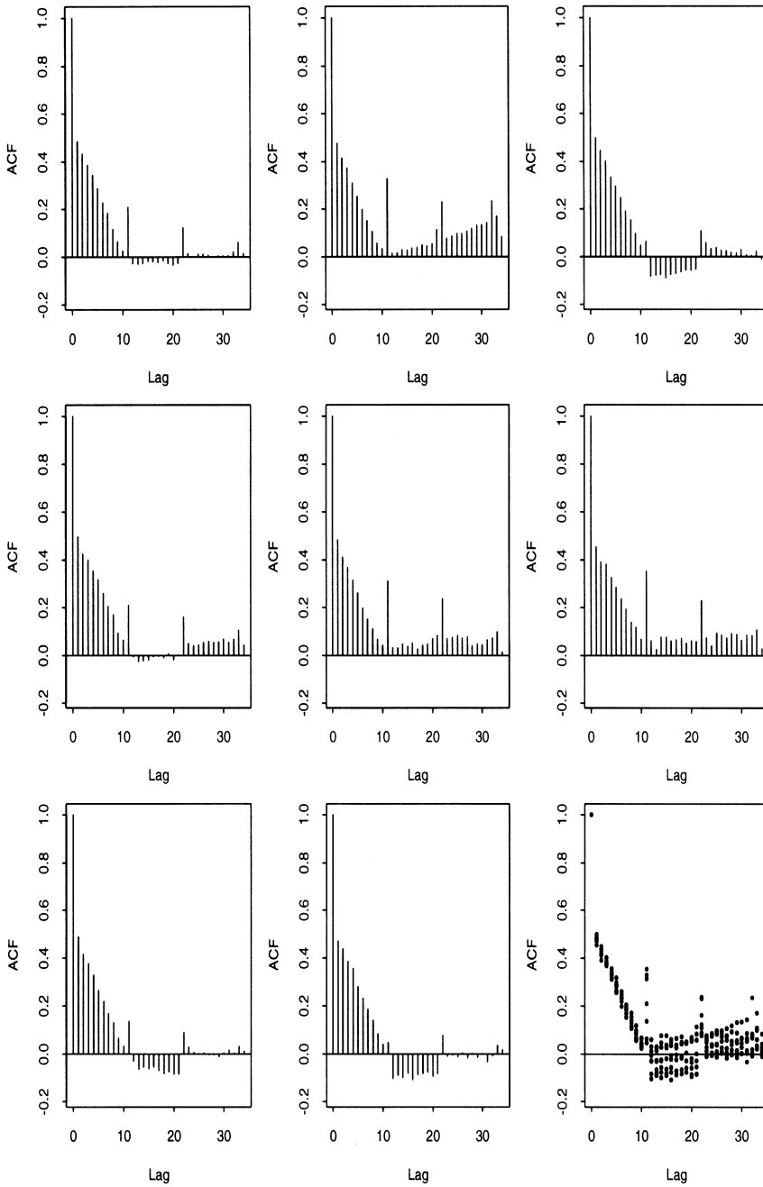
FIG. 1. Stable moving average: sample correlation functions.
