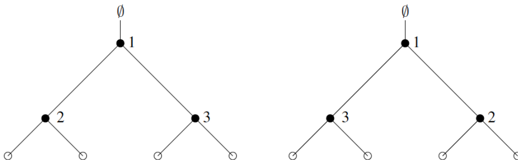
Figure 2: The only two possible monotonous numberings for the tree on the right of Figure 1. The left tree there admits only one such numbering.
