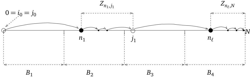
FIGURE 1. A typical configuration which contributes to \widehat{Z}_\omega^{(i_1, \dots, i_\ell)} defined in (3.10). In this example we have a number N/k = 4 of blocks, \ell = 2 and i_1 = 2 , while i_\ell = N/k = 4 by definition (cf. (3.9)). Big black dots denote the n_i 's, white dots denote the j_i 's, while small dots are all the other points of \tau . Note that j_1 - n_1 < k , as it should, and that there is no point of \tau between a white dot and the next big black dot. In this example, the set M of (3.14) is \{2, 3, 4\} , and as a consequence W defined in (3.15) is B_2 \cup B_3 \cup B_4 . In words: n_1 is the first point of \tau after 0, j_1 is the last point of \tau which does not exceed n_1 + k - 1 , n_2 is the first point after j_1 , and so on. The index of the block containing n_r defines i_r .
