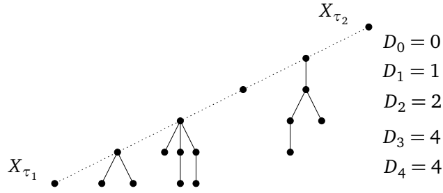
Figure 4: For the path in Figure 3 the process (D_k)_{k \geq 0} is realized as (0, 1, 2, 4, 4, 0, \dots) . The solid lines represent downcrossings. The thick dots on the dashed line correspond to the single immigrant in definition (32).
