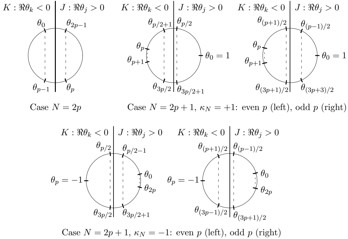
Figure 1: The N^{\text{th}} roots of \kappa_N
