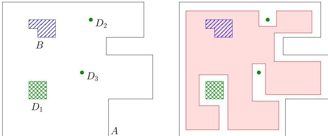
Figure 1: An illustration of Lemma 2. On the left, a simple rational polyomino A , containing in its interior simple rational polyominoes B and D_1 , and singletons D_2 and D_3 . On the right, a simple rational polyomino C (shaded) within the interior of A that contains B and avoids D_1, D_2, D_3 .
