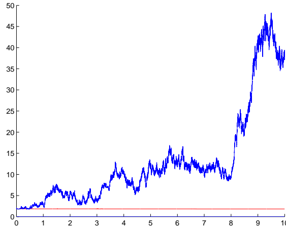
Figure 1: The process f(Z, W) (red) and the square radial process Z\bar{Z} + W\bar{W} (blue) for the example above
