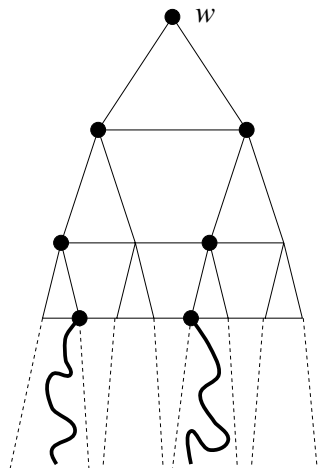
Figure 2: The infinite black clusters separate.
