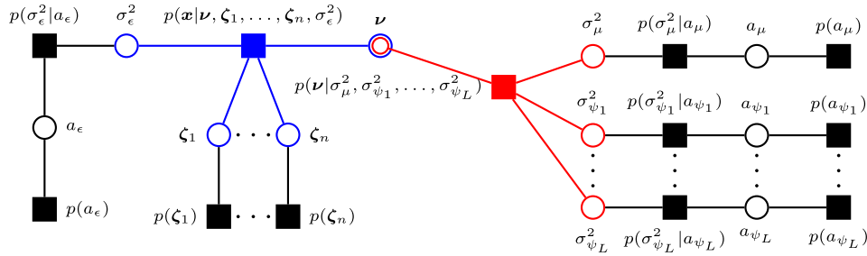
Figure 1: The factor graph for the Bayesian FPCA model in (2.6).
