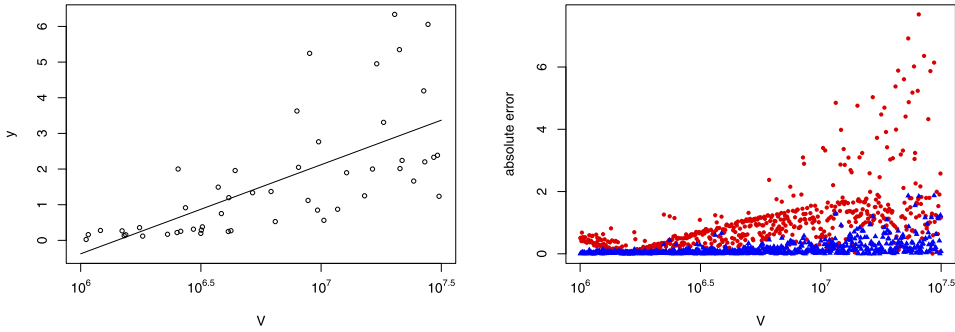
FIG. 4. The left figure is the least squares fit of simulator output to volume for 50 simulator runs at a specific location. The right figure compares use of this least squares fit to estimate the outputs of 633 other simulator runs (the red dots), corresponding to other input values at the same location, with use of the PP GaSP (developed from the same 50 simulator runs) to estimate the 633 outputs (the blue triangles). Accuracy is measured by the absolute error of the prediction |y(x_i^*) - \hat{y}(x_i^*)| .
