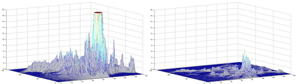
FIG. 1. Median (truncated at 20 meters at the volcanic center region) and interquartile range of the GaSP emulator of “maximum flow height over time” for TITAN2D, at 23,040 spatial locations over Montserrat Island and for new input values V^* = 10^{6.9984} , \varphi^* = 3.3487 , \delta_{\text{bed}}^* = 10.8790 and \delta_{\text{int}}^* = 31.0300 .
