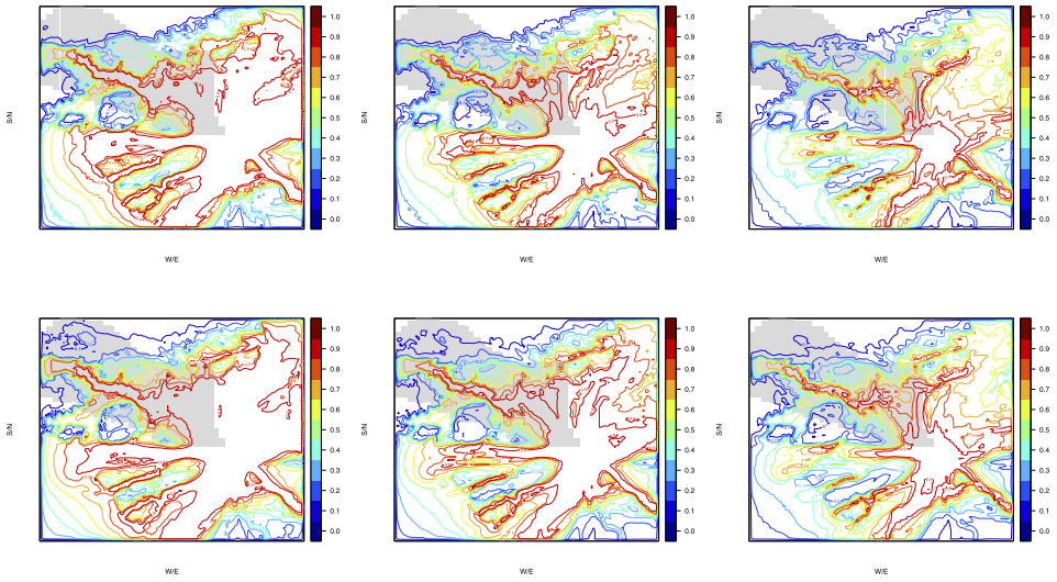
FIG. 3. For SHV, contours of the probabilities that the maximum flow heights exceed 0.5 (left), 1 (center) and 2 (right) meters over the next T = 2.5 years at each location on SHV. The shaded area is Belham Valley, which is still inhabited. The results in the upper row utilized only N = 50 runs of TITAN2D to construct the PP GaSP, while the lower row results were based on utilizing all N = 2048 runs.
