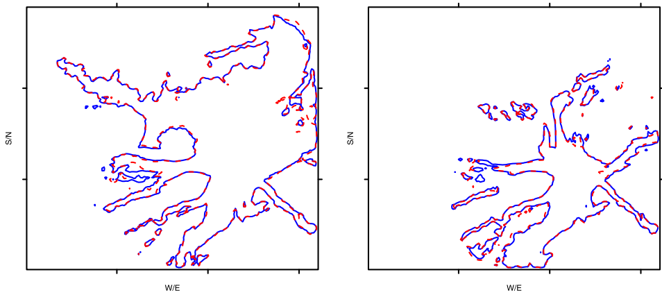
FIG. 2. 1 m spatial contours of maximum pyroclastic flow height on Montserrat Island for two held-out values of the inputs. The red dashed contour is from the actual simulator run, while the blue solid contour is the prediction from the PP GaSP emulator with 3 inputs ( V , \delta_{\text{bed}} , \phi ) and an estimated nugget. The held-out testing inputs for the left figure are V^* = 10^{7.1368} , \varphi^* = 1.8484 , \delta_{\text{bed}}^* = 12.2940 and \delta_{\text{int}}^* = 24.2140 . Those for the right figure are V^* = 10^{6.8292} , \varphi^* = 4.5360 , \delta_{\text{bed}}^* = 12.7880 and \delta_{\text{int}}^* = 27.3000 .
