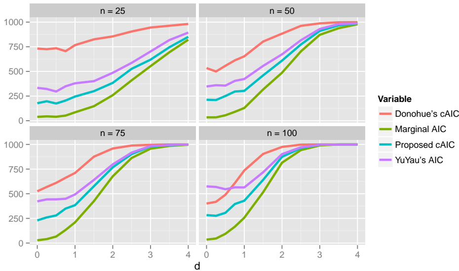
FIG 3. Results for the spline smoothing model with exponentially distributed responses. The y-axis shows the number of simulation replications where out of 1000 the more complex model was favoured by the different AICs.
