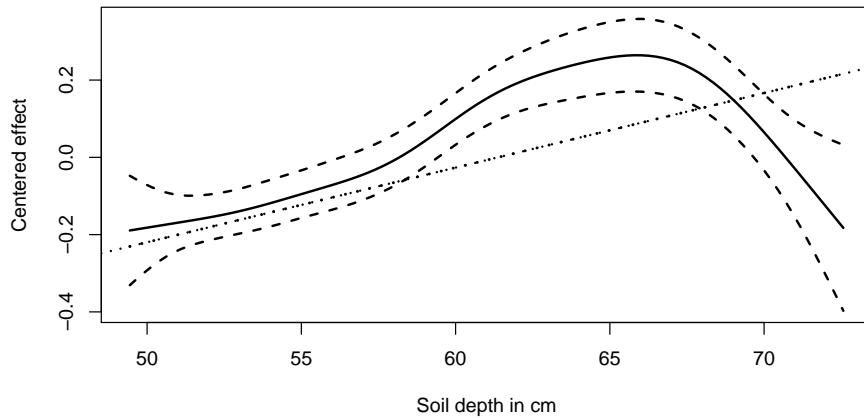
FIG 5. The linear effect (dotted line) and the nonlinear effect (solid line) with confidence interval (dashed lines) of the soil depth on the tree growth. The pointwise confidence intervals are defined using twice the standard deviation of the estimator.
