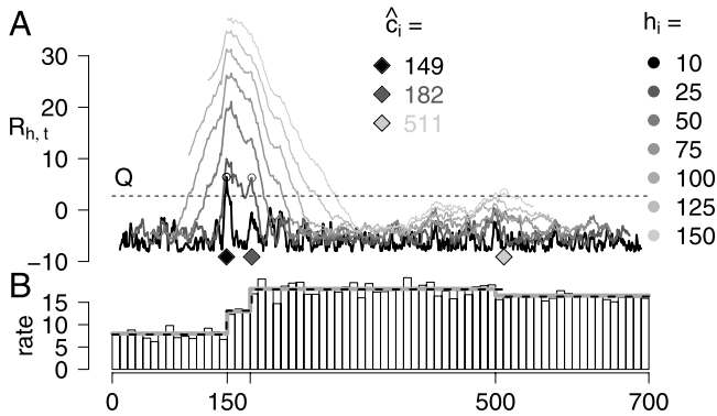
FIG. 7. Application of the MFT to a simulated point process on (0, 700] with three change points at c_1 = 150, c_2 = 180 and c_3 = 500 . The life time distributions were \exp(8) in [0, c_1] , \Gamma(2, 26) in [c_1, c_2] , \exp(18) in [c_2, c_3] and \Gamma(2, 33) in [c_3, T] , corresponding to rates of 8, 13, 18 and 16.5 in the respective intervals. (A) Gray curves indicate the processes (R_{h,t}) for window sizes h \in H = \{10, 25, 50, 75, 100, 125, 150\} . The simulated threshold Q = 2.75 is indicated by the dashed line. The estimated change points \hat{c}_1 = 149, \hat{c}_2 = 182, \hat{c}_3 = 511 are marked by diamonds. As indicated by the grayscale of the diamonds, each change point was detected by a different window size. (B) Rate histogram of the underlying point process with real (gray) and estimated (dashed) rate profiles.
