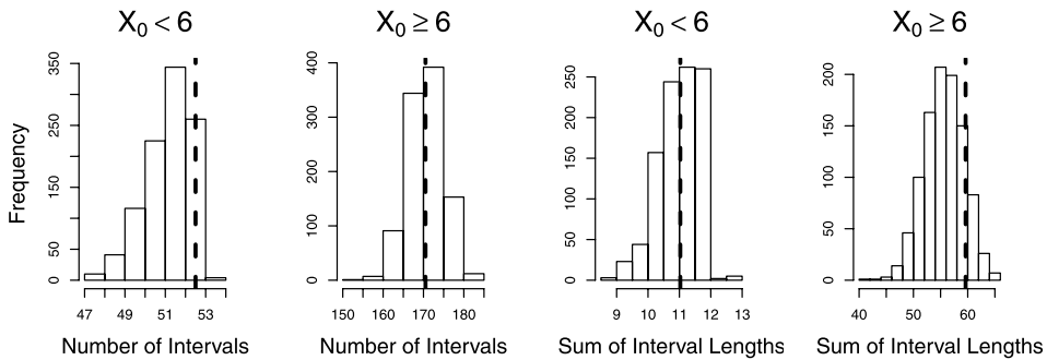
FIG. 3. Low- vs high-count genotype analysis. Histograms of simulated numbers of intervals and sums of interval lengths are plotted for intervals with starting values less than six and greater or equal to six. The vertical dashed lines indicate the observed values of the four statistics.
