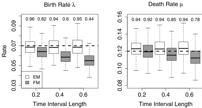
FIG. 1. Box plots of birth (left panel) and death (right panel) rate estimates, obtained from 200 simulated data sets using the EM algorithm and frequent monitoring (FM) method. The true parameter values, used in data simulations, are marked by the horizontal dashed lines. Above the box plots, we show Monte Carlo estimates of coverage probabilities of the 95% confidence intervals.
