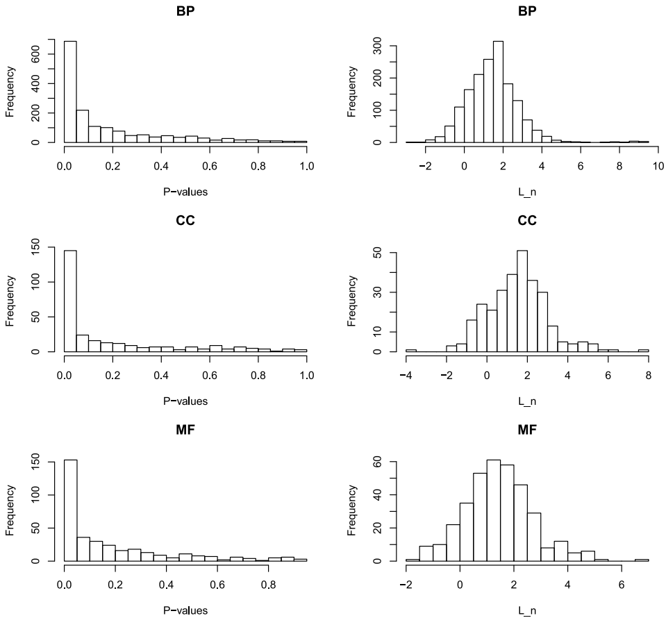
FIG. 1. Histograms of p -values (left panels) for testing two covariance matrices and test statistic L_n (right panels) for the three gene-categories.
