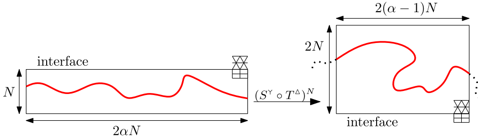
FIG. 9. Transformation of a horizontal crossing of B_{\alpha N, N} by (S^\vee \circ T^\Delta)^N . The interface moves down N steps. The path drifts by at most distance N and cannot go below the interface of the image lattice.
