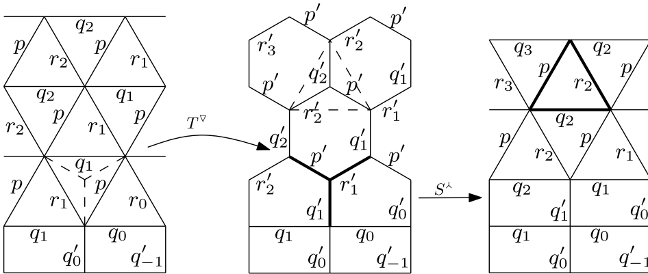
FIG. 15. Left: The measure \mathbb{P}_{\mathbf{q},\mathbf{r},p} on \mathbb{L} . In the triangular part the measure is \mathbb{P}_{p,\mathbf{q},\mathbf{r}}^\Delta on a rotated lattice, and in the square part it is \mathbb{P}_{\mathbf{q},\mathbf{q}'}^\square . Middle, right: Application of S^\lambda \circ T^\nabla transforms \mathbb{L} to a copy of itself shifted upward and sideways.
