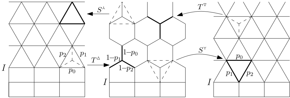
FIG. 6. Transformations S^\lambda , S^\gamma , T^\Delta and T^\nabla of mixed lattices. The transformations map the zones with dashes to the bold triangles/stars. The interface-height decreases by 1 from the leftmost to the rightmost graph.
