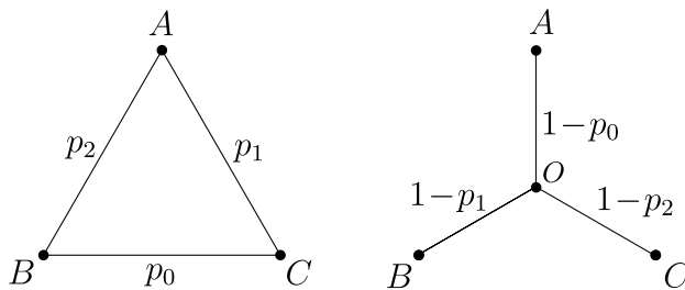
FIG. 4. The star–triangle transformation.
