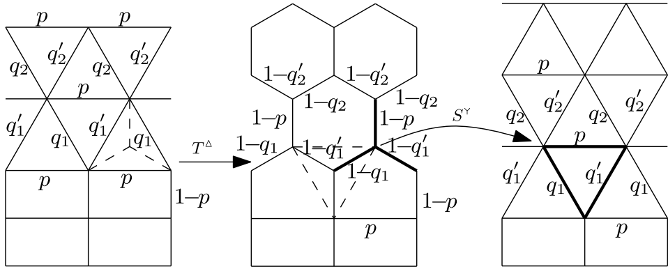
FIG. 14. A mixed triangular lattice (left) with the highly inhomogeneous measure above the interface. The transformation S^Y \circ T^\Delta moves the interface down by one unit. Every triangle is parametrized by a self-dual triplet.
