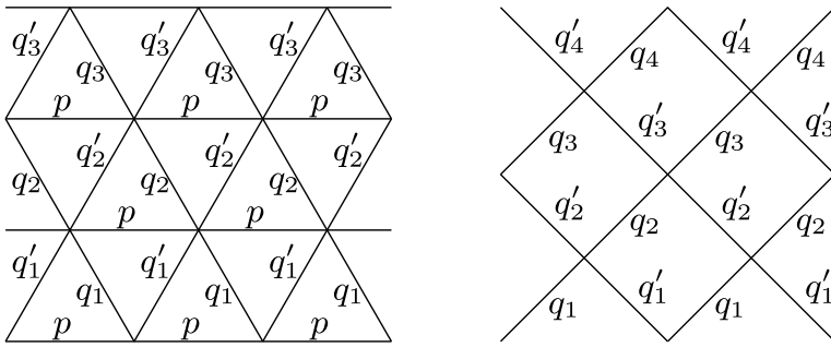
FIG. 2. Left: The triangular lattice with the highly inhomogeneous product measure \mathbb{P}_{p, \mathbf{q}, \mathbf{q}' }^\Delta . The probability for each edge to be open is described in the picture: all horizontal edges have probability p of being open, while the other edges have probability q_n (right edges of upward pointing triangles) or q'_n (left edges of upward pointing triangles) of being open, with n being their height. Right: The square lattice with a highly inhomogeneous product measure \mathbb{P}_{\mathbf{q}, \mathbf{q}' }^\square , rotated by \pi/4 . Edges inclined at angle \pi/4 have probability q_n of being open, while edges inclined at angle 3\pi/4 have probability q'_n of being open, with n being their height.
