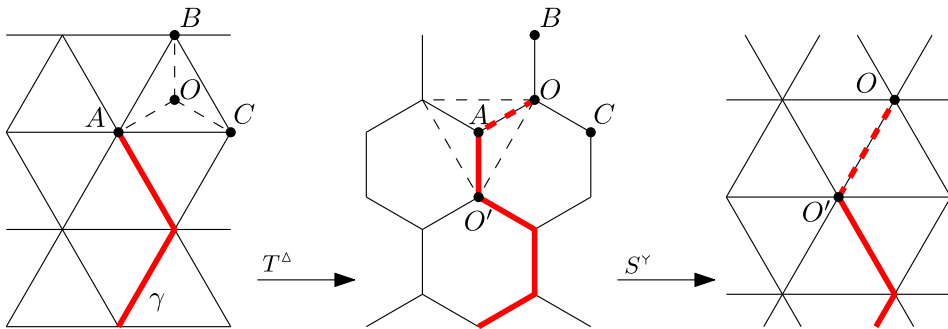
FIG. 10. An illustration of the action of S^\gamma \circ T^\Delta when \Gamma^k = \gamma . The top endpoint A of \gamma is preserved under T^\Delta . If \omega^k(BC) = 0 , there is a strictly positive probability that AO is open in T^\Delta(\omega^k) , in which case h^{k+1} \geq h^k + \frac{1}{2} .
