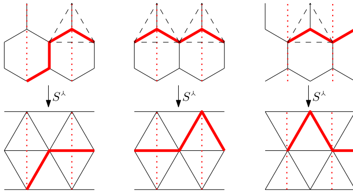
FIG. 12. Three examples of growth of path-height within a column under the action of S^\lambda , under the assumption H_n(\Gamma_k) \geq \max\{H_{n-1}(\Gamma_k), H_{n+1}(\Gamma_k)\} . Left: The base of the marked triangle is present in the image, and the height does not increase. Middle: The base of the rightmost marked triangle is absent. The heights in the central and right columns increase. There is a strictly positive probability that both marked bases are present, and that the height in the central column does not increase. Right: The base of the marked triangle is absent, and the height increases by 1.
