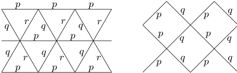
FIG. 3. Each graph, when repeated periodically, constitutes a model included within the analysis of highly inhomogeneous models. Left: A triangular-lattice model with a horizontal axis of symmetry, as in [18], Section 2.1. Right: A variant on the square-lattice model.
