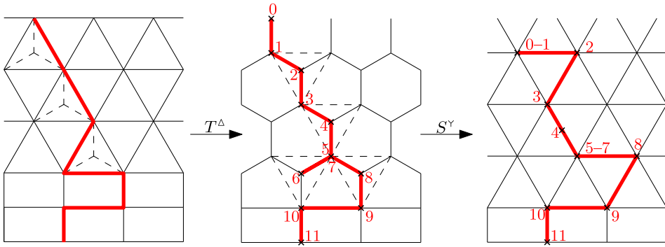
FIG. 7. Transformations of lattice-paths. The transformation T^\Delta acts deterministically on open paths, each edge of a triangle being transformed into two segments of an upward pointing star. When applying S^\Upsilon , the segment labeled from 0 to 1 contracts to one point, as does that labeled from 5 to 7.
