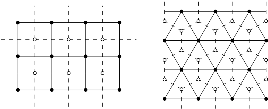
FIG. 1. The square lattice and its dual square lattice. The triangular lattice and its dual hexagonal lattice.
