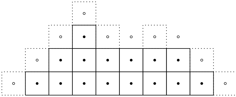
FIG. 13. The solid squares represent the bricks at step k in the growth process. The dotted squares are the additions at time k + 1 . The lateral extensions occur with probability 1, and the vertical extensions with probability 1 - \zeta .
