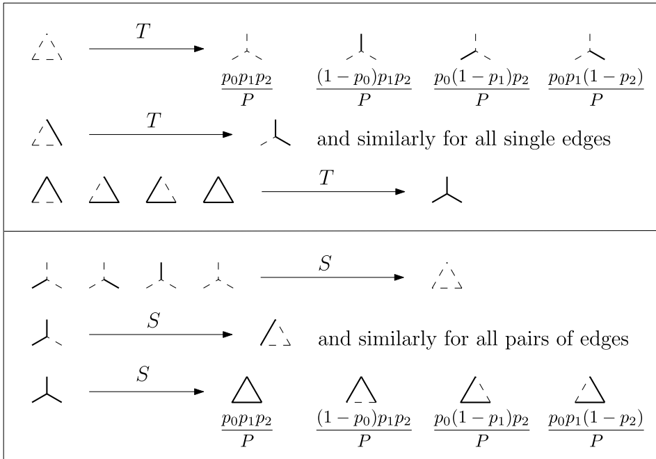
FIG. 5. The “kernels” T and S and their transition probabilities, with P := (1 - p_0)(1 - p_1) \times (1 - p_2) . Since \kappa_{\Delta}(\mathbf{p}) = 0 , the probabilities in the first and last rows sum to 1.
