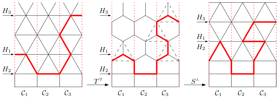
FIG. 11. The evolution of the heights of a crossing within columns, when applying T^\nabla and S^\wedge . The heights in each column are the same in the first and second lattice. In the third, H_1 increases by 1; H_2 increases by 2; H_3 does not change.
