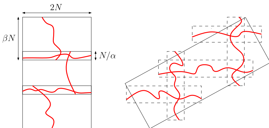
FIG. 8. Left: Vertical crossings of copies of B_{N,\beta N} and horizontal crossings of copies of B_{N,N/\alpha} , for large \alpha , may be combined to obtain vertical crossings of boxes with arbitrary aspect ratio. Right: Crossings of the type C_h(\gamma n, n) and C_v(n, \gamma n) may be combined to obtain crossings of boxes with general inclination.
