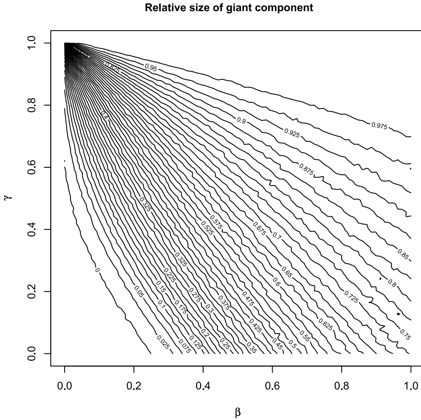
FIG. 3. Simulation of the proportion of vertices in the giant component in the linear case. The curve forming the lower envelope is determined explicitly in Proposition 1.3. The plot is based on 15,000 Monte Carlo simulations of the branching process for 80 times 80 gridpoints in the (\beta, \gamma) -plane.
