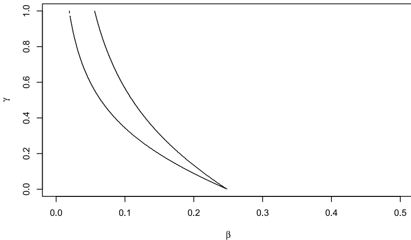
FIG. 4. For the attachment function f(k) = \gamma\sqrt{k} + \beta the figure shows the curves a[f] = \frac{1}{2} and a[f] + \sqrt{a[f]c[f]} = 1 , which form lower and upper bound for the boundary between the two phases, nonexistence and existence of the giant component, in the (\beta, \gamma) -plane.
