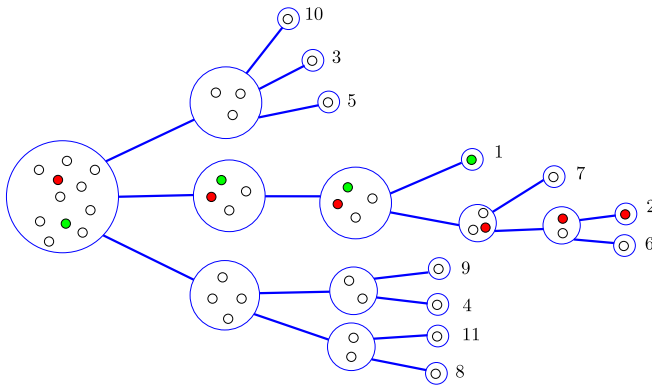
FIG. 2. A sample tree T_{[n]} for n = 11 , with the labeled leaves. The process \Pi^{(11)} can be easily deduced: for instance, \Pi^{(11)}(1) = \{\{1, 2, 6, 7\}, \{3, 5, 10\}, \{4, 8, 9, 11\}\} . As opposed to Figure 1, leaves are all connected to vertices with at least 2 children, because of the requirement q_1(\emptyset) = 1 .
