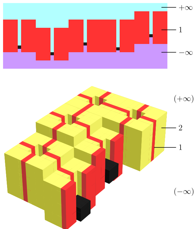
FIG. 2. Part of the random coloring \lambda of Proposition 8, for d = 2 (top), and d = 3 (bottom, with colors \pm\infty shown as transparent). Holes are shown as black.
