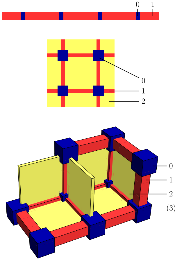
FIG. 1. Part of the coloring \alpha of Lemma 10, for d = 1 (top), d = 2 (middle), d = 3 (bottom; color 3 is shown as transparent, and only selected slabs are shown).
