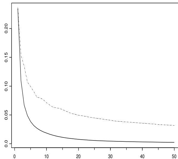
Figure 8: Random walk with k = 5 , p = 0.5 , \epsilon = 0.1 and N = 1, \dots, 500000 , depicted at every 10000th iteration: \hat{\sigma}_{\max, N} under Method 1 (solid line) and \tilde{\sigma}_{\max, N} under Method 2 (dashed line).
