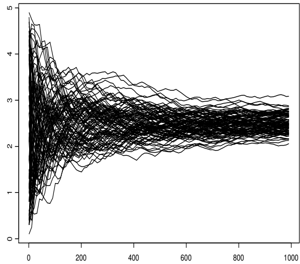
Figure 3: Random walk with k = 5 and p = 0.5 . One hundred independent simulations of the running mean over 1000 iterations.
