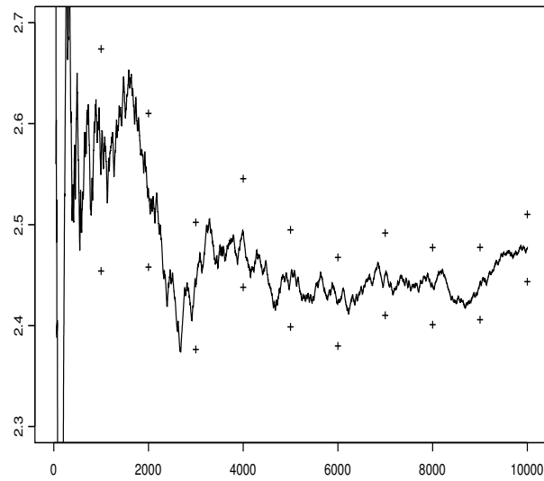
Figure 5: Random walk with k = 5 and p = 0.5 . Conservative 95% confidence bounds (indicated by crosses) on the running mean when t = 1, \dots, 10000 and Method 1 is used.
