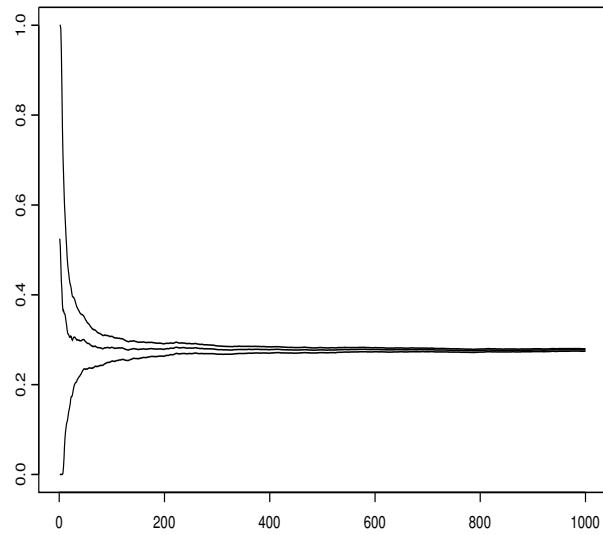
Figure 11: Mixture model with p = 0.3 and normal distributions N(0, 1) and N(2, 1) . Running mean and upper and lower bounds for N = 1000 .
