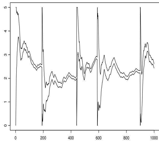
Figure 6: Random walk with k = 5 and p = 0.5 . Method 2 for obtaining L_t^{(i)} and U_t^{(i)} when t = 1, \dots, 1000 .
