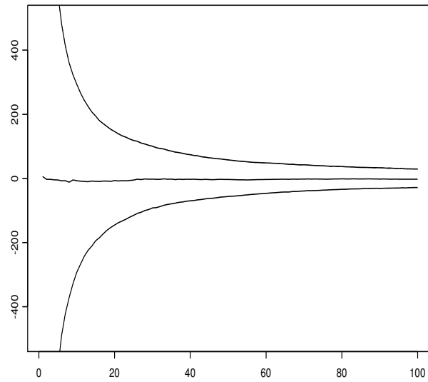
Figure 9: Method 1 for an Ising model with M = 64 and \beta = 0.1 . Running mean \bar{\phi}_t and upper and lower bounds \bar{\phi}_t^U and \bar{\phi}_t^L .
