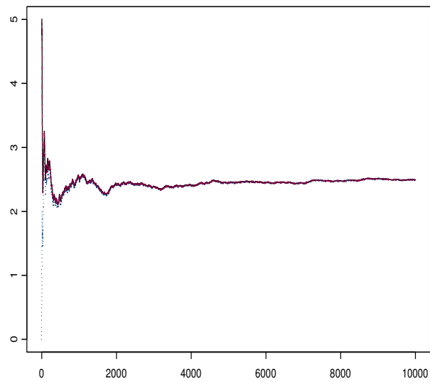
Figure 1: Random walk with k = 5 and p = 0.5 . Running mean and upper and lower bounds over 10000 iterations.
