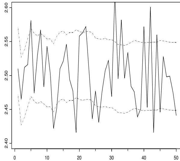
Figure 7: Random walk with k = 5 , p = 0.5 , \epsilon = 0.1 and N = 1, \dots, 500000 , depicted at every 10000th iteration: \bar{\phi}_N^L and \bar{\phi}_N^U under Method 1 (solid line) and \tilde{\phi}_N^L and \tilde{\phi}_N^U under Method 2 (dashed lines). Note that \bar{\phi}_N^L and \tilde{\phi}_N^L are effectively equal for these values of N .
