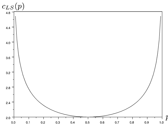
FIG. 2. The graph of p \mapsto c_{\text{LS}}(p) .
