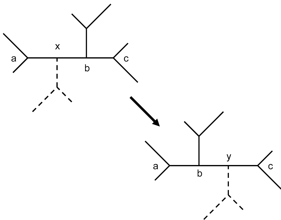
FIG. 1. An SPR move. The dashed subtree tree attached to vertex x in the top tree is reattached at a new vertex y that is inserted into the edge (b, c) in the bottom tree to make two edges (b, y) and (y, c) . The two edges (a, x) and (b, x) in the top tree are merged into a single edge (a, b) in the bottom tree.
