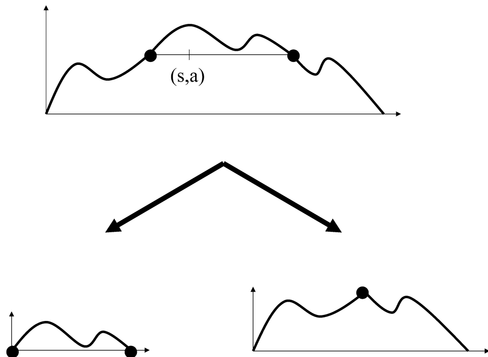
FIG. 3. The decomposition of the excursion e (top picture) into the excursion \hat{e}^{s,a} above level a that straddles time s (bottom left picture) and the “remaining” excursion \check{e}^{s,a} (bottom right picture).
