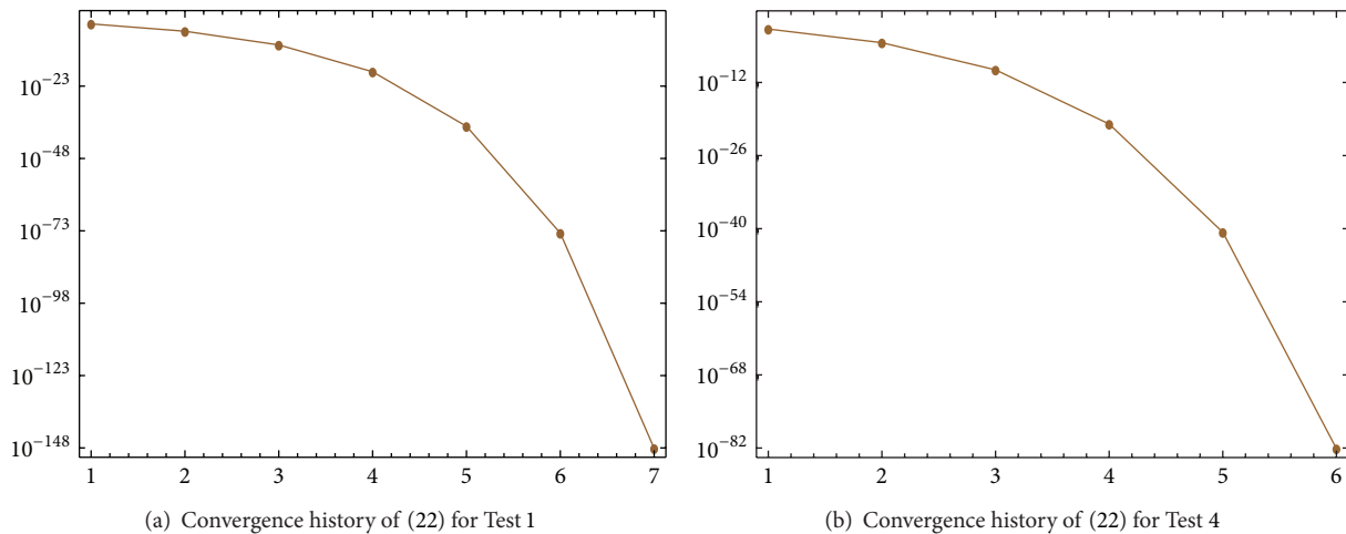
FIGURE 4: Using \beta = 0.0001 in (22) so as to solve different tests.
