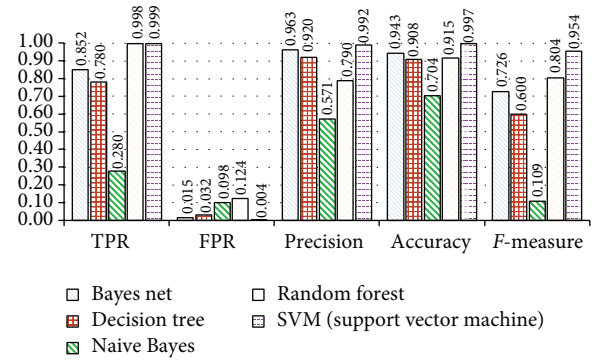
FIGURE 6: Detection results of respective classifiers.
