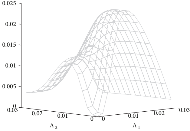
FIGURE 7: We illustrate here the dependence of P_{\Lambda}(\bar{\lambda}_0, \bar{X}_0) as a function of the exercise boundary \Lambda ; this allows to find the optimal ( \Lambda_1^* = 121 bps, \Lambda_2^* = 0 ) that maximizes the option price.
