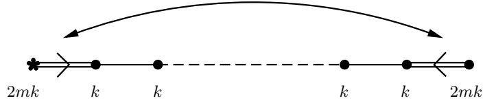
Figure 5. Spectral diagram for R_0=C_n and X=Q(R_0) .
