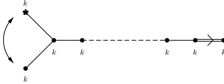
Figure 2. Spectral diagram of the Iwahori–Hecke algebra of \mathrm{Sp}_{2n}(F) .
