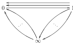
Figure 2. Modified quiver
