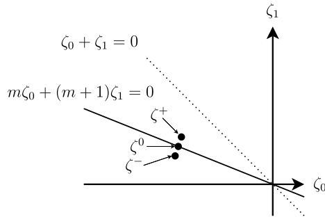
Figure 3. Wall-crossing
