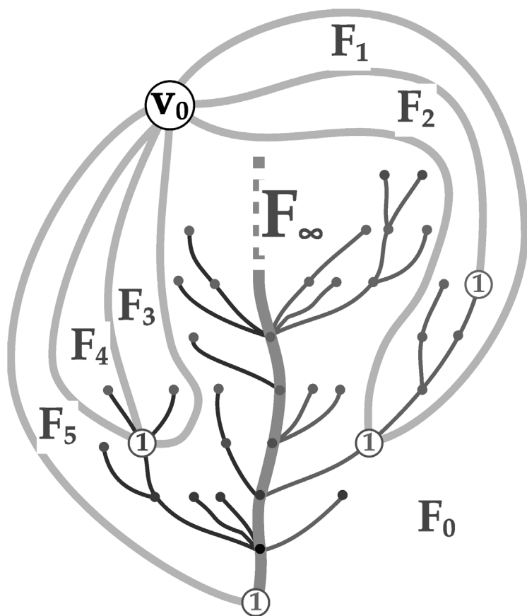
FIG. 4. Step 1, leading to finite faces F_i, 0 \leq i \leq 5 , and the infinite face F_\infty .
