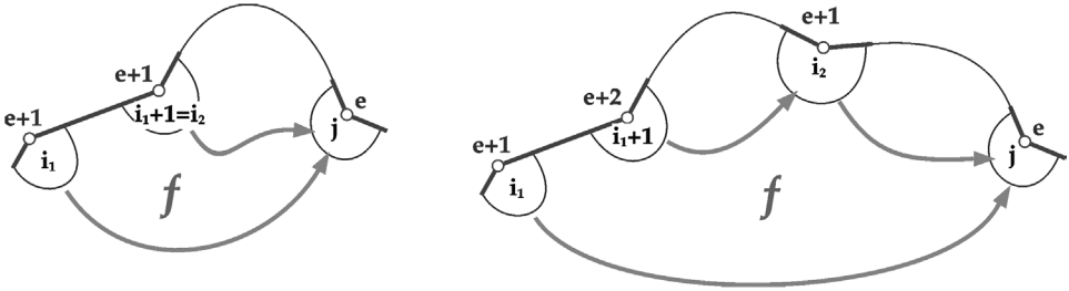
FIG. 7. Two possible sizes for f : triangular or quadrangular.
