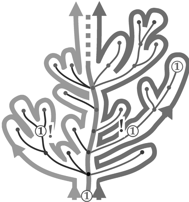
FIG. 3. Contour traversal (a) of the left side and (b) of the right side of the spine. The last occurrence of label 1 is signaled by an exclamation mark.
