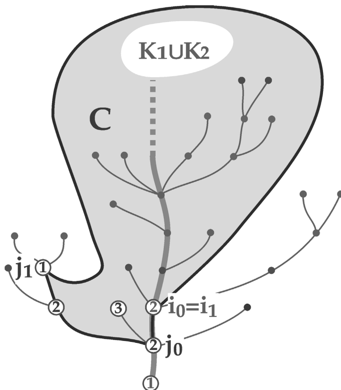
FIG. 8. The closed curve C for R = 2 .
