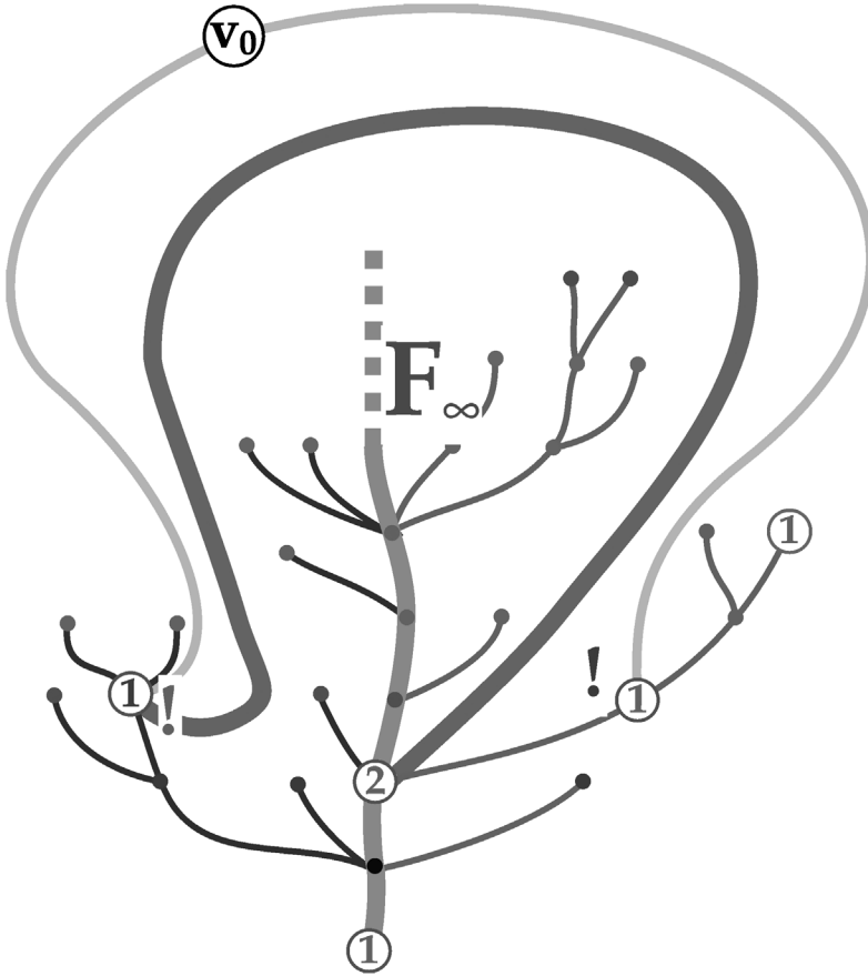
FIG. 6. Inside F_\infty , a chord that joins two sides of the spine, with \ell(2) = 2 , \ell(-1) = 1 and s(2) = -1 \triangleright 2 .
