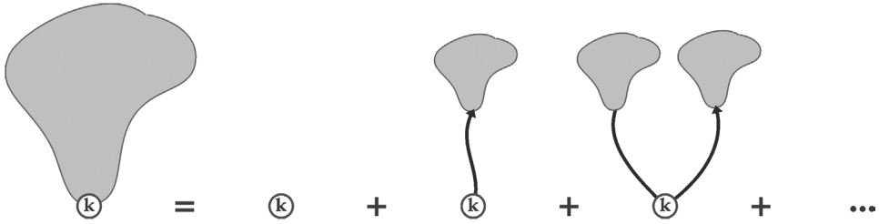
FIG. 1. Decomposing a tree: W^{(k)} = \frac{1}{1-Z^{(k)}} .
