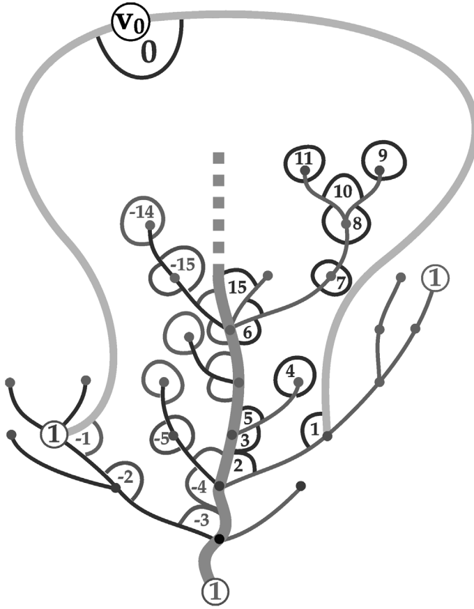
FIG. 5. Numbering the corners of the infinite face.
