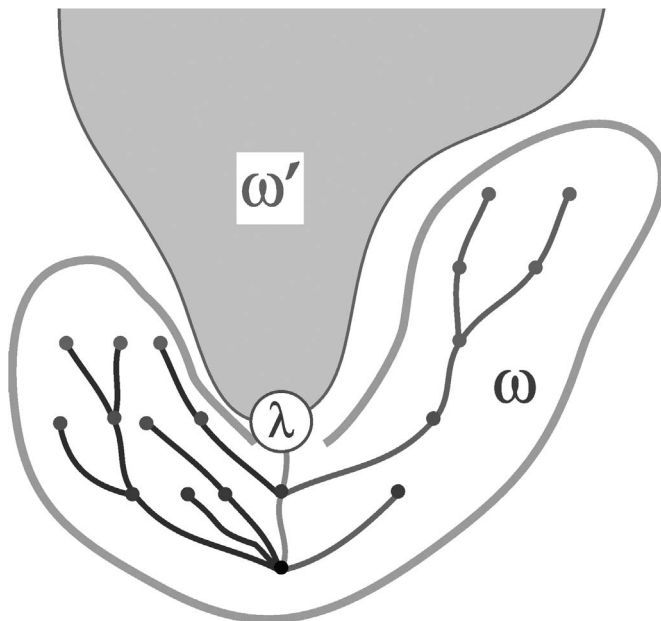
FIG. 2. Grafting a tree: \text{gr}(\omega, \lambda, \omega') .
