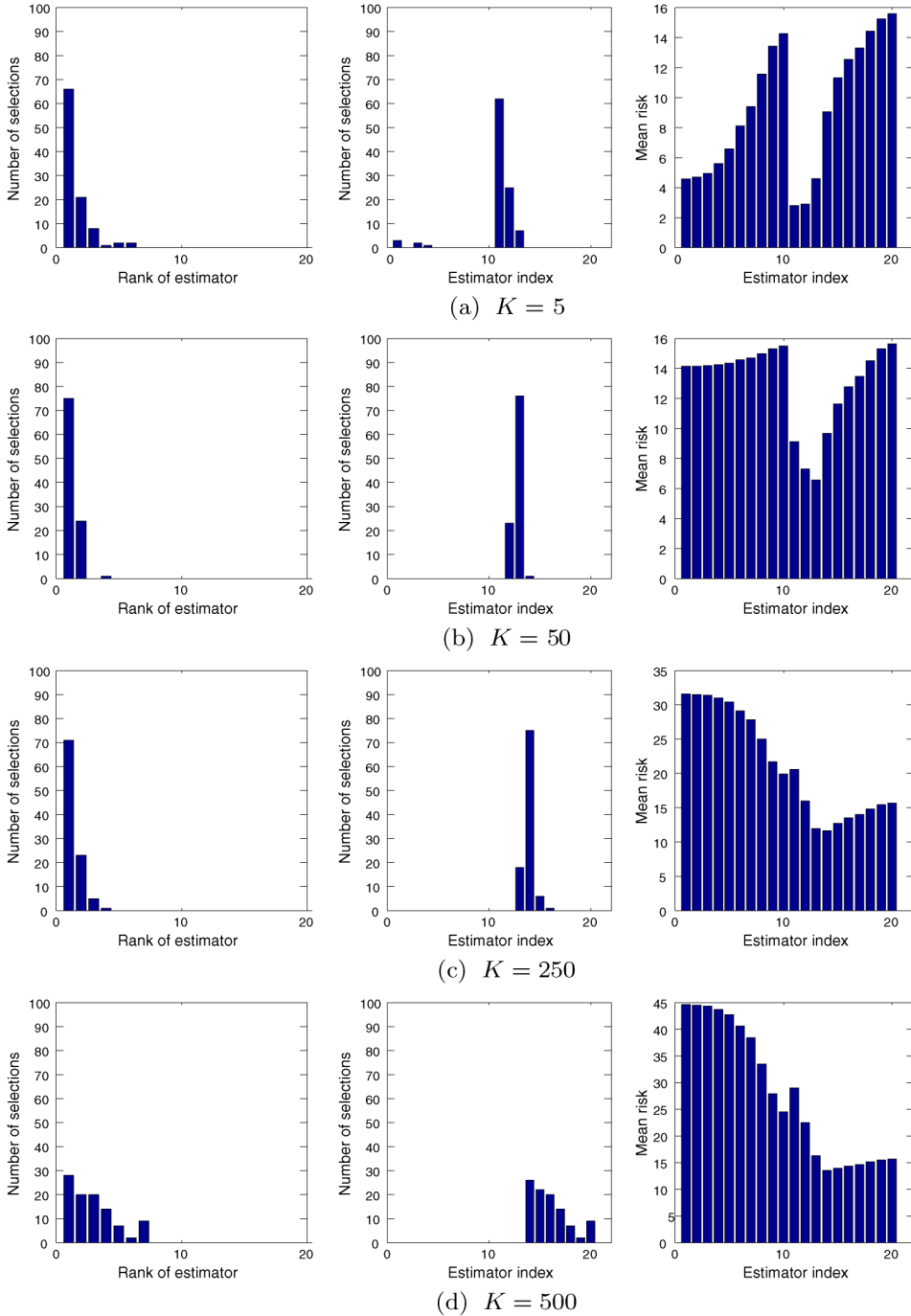
FIG. 1. Scenario (i). Left column: the number of replications out of 100 where the procedure selects the estimator with rank 1, 2, . . . , 20. Middle column: the number of selections versus the estimator index. Right column: the average \mathbb{L}_2 -risk versus the estimator index. Sparsity parameter K : (a) K = 5 ; (b) K = 50 ; (c) K = 250 ; (d) K = 500 .
