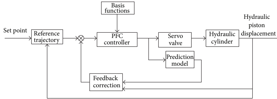
FIGURE 1: Block scheme of predictive function control (PFC).
