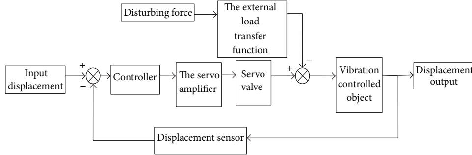
FIGURE 2: Block scheme of the hydraulic servo control system.
