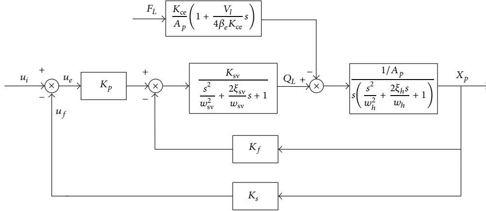
FIGURE 3: Block scheme of the hydraulic servo system.
