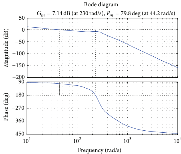
FIGURE 4: The amplitude and phase frequency characteristics of the servo system.
