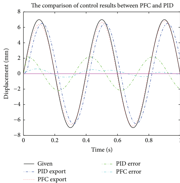
FIGURE 6: Comparison of PFC and PID control simulation results.
