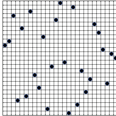
Figure 1: An example of a Costas array of order 27: note the haphazard positioning of its dots.
