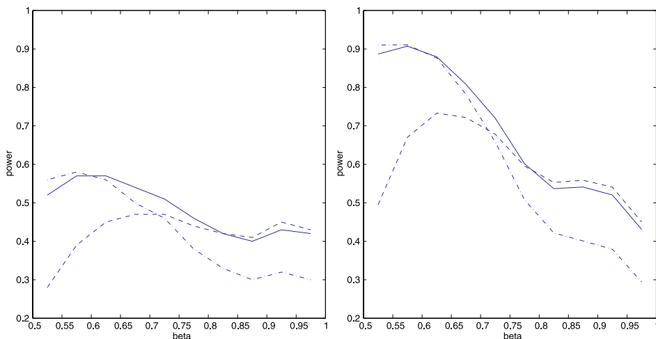
FIG 2. Power of ALR_n (solid), HC_n^* (dashed) and BJ_n^+ (dash-dot) as a function of the sparsity parameter \beta . The left plot shows power for sample size n = 10^4 , the right plot for n = 10^6 .
