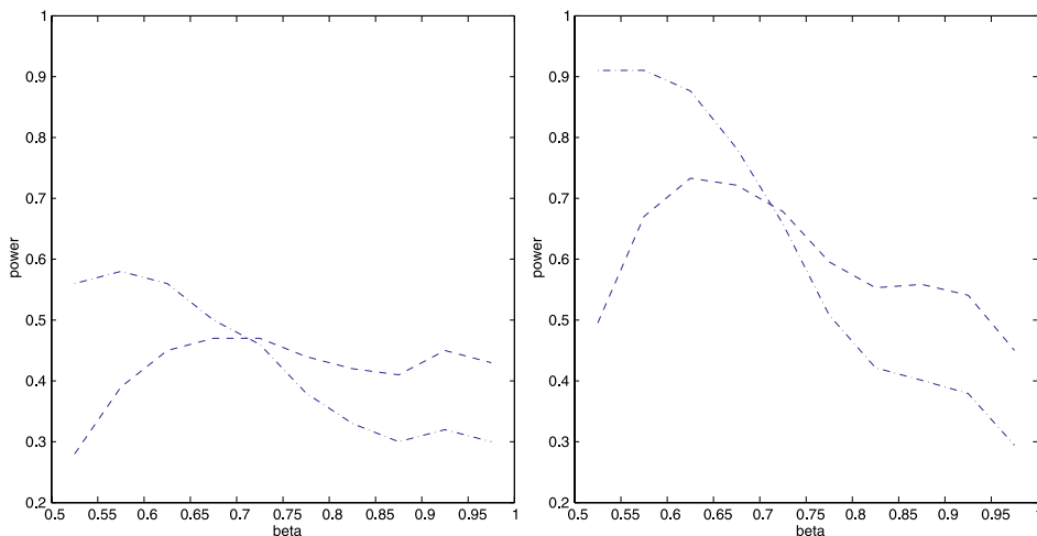
FIG 1. Power of HC_n^* (dashed) and BJ_n^+ (dash-dot) as a function of the sparsity parameter \beta . The left plot shows power for sample size n = 10^4 , the right plot for n = 10^6 .
