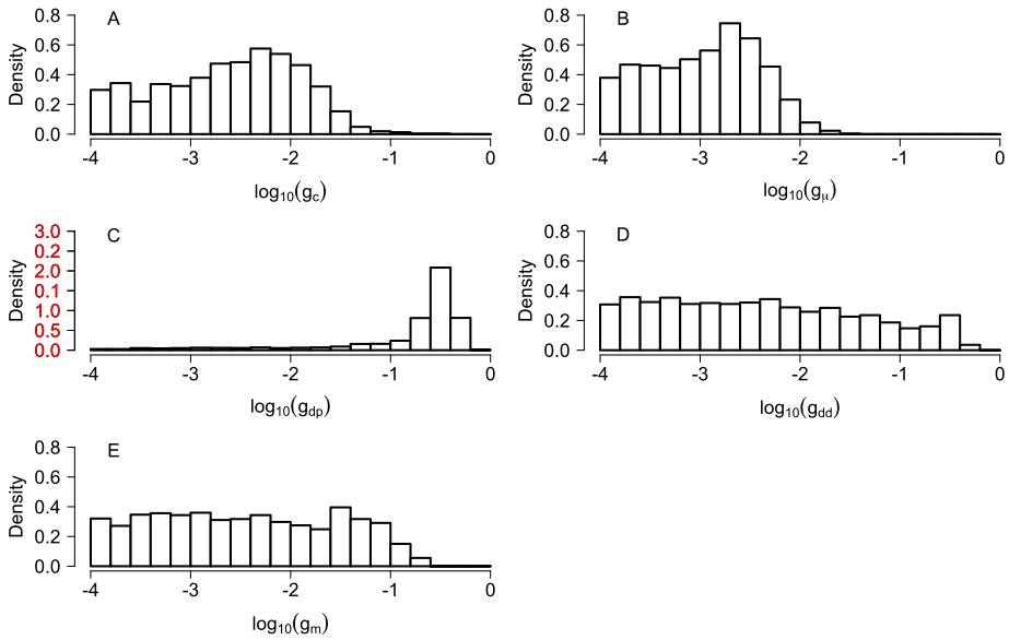
FIG. 4. Posterior distributions of \log_{10} g for the FMR1 data. g in (A)–(D) is the scaled variance in the beta distribution assumed for (A) measurement error rate c (due to inappropriate bisulfite conversion); (B) failure of maintenance rate 1 - \mu ; (C) parent de novo rate \delta_p ; and (D) daughter de novo rate \delta_d . In (E), g_m reflects deviation from the stationarity assumption. See Table 3 for guidelines on the interpretation of values of \log_{10} g . The y-axis in (C) has a wide range.
