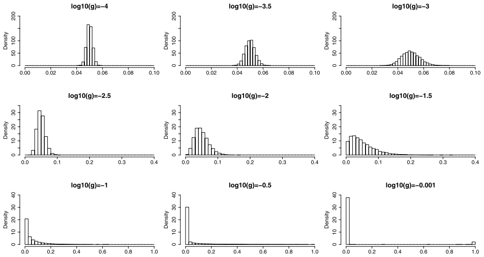
FIG. 2. Shape of a beta distribution changes with respect to scaled variance g . Data were simulated for beta distributions with mean r = 0.05 and different values of scaled variance g . Ranges of the horizontal and the vertical axes are different between rows. As g increases, the histogram spreads out to the entire support of (0, 1) and a second peak at 1 starts to appear (bottom right panel).
