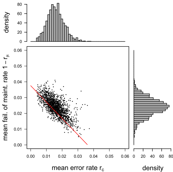
FIG. 3. Posterior distributions and scatter plot of mean failure of maintenance rate, 1 - r_\mu , and mean error rate, r_c , under the multi-site model for the FMR1 data. The red line, 1 - \mu = 1.04c + 0.04 , indicates a predicted relationship for these estimates under a much simpler analysis (see Section 3.2).
