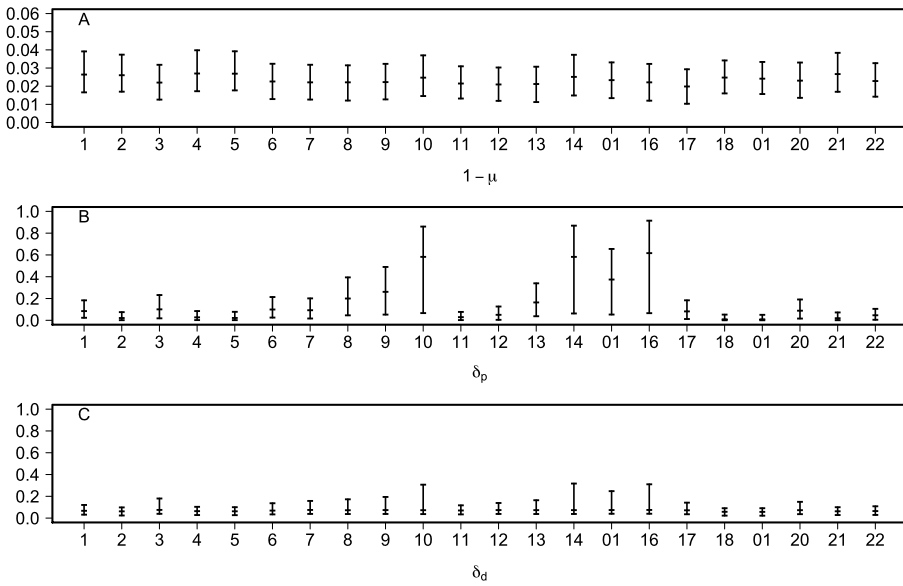
FIG. 6. Median and 80% credible intervals of CpG-site-specific estimates of (A) failure of maintenance rates 1 - \mu , (B) parent de novo rates \delta_p and (C) daughter de novo rates \delta_d under the multi-site model for the FMRI data. The numbering of the CpG sites follows the convention established in Stöger et al. (1997).
