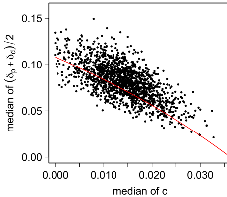
FIG. 7. Joint posterior distribution of the median of the average of the parent and daughter de novo rates, (\delta_p + \delta_d)/2 , and the median of the error rate c for the FMRI data. The red curve, (\delta_p + \delta_d)/2 = 0.44 + 0.05/(c - 0.15) , indicates a predicted relationship for these estimates under a much simpler analysis (see text).
