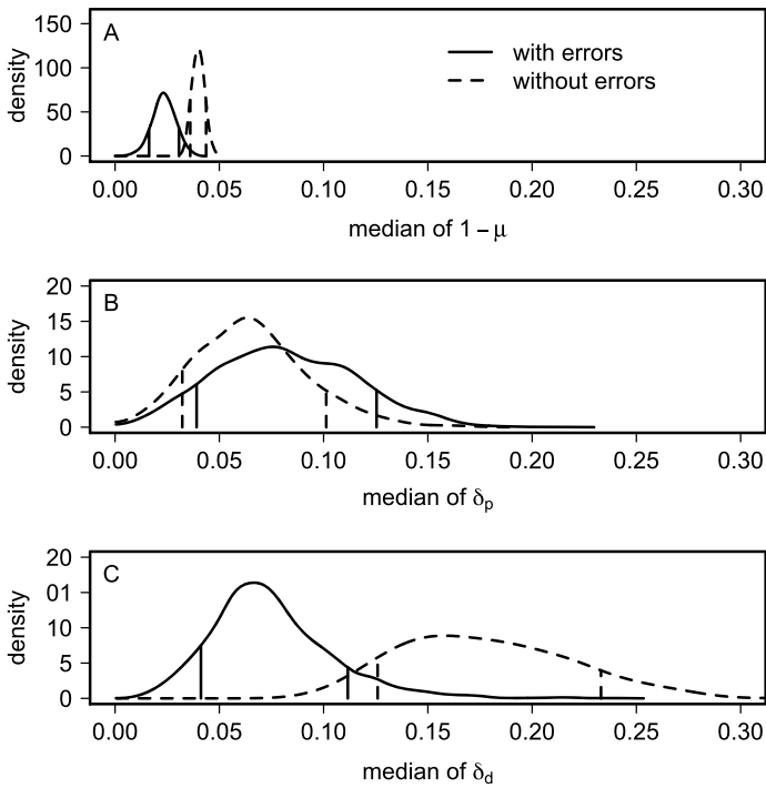
FIG. 8. Impact of measurement errors (due mainly to inappropriate bisulfite conversion error) on the inference of the rates of methylation events. Solid lines incorporate these errors, whereas dashed lines do not. From top to bottom are posterior densities of medians of (A) failure of maintenance rate 1 - \mu , (B) parent de novo rate \delta_p and (C) daughter de novo rate \delta_d . Vertical bars indicate the 80% credible interval (10% and 90% percentiles) for each density.
