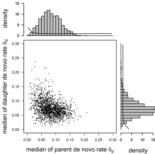
FIG. 5. Posterior distributions and scatter plot of median de novo rates \delta_p and \delta_d under the multi-site model for the FMR1 data. Smooth curves in the histograms are density functions of the median of 22 beta random variables, each corresponding to a parent (or daughter) de novo rate at a CpG site. The two density curves are identical because the prior distributions for the rates are identical.
