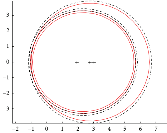
FIGURE 1: The red dotted line and black dashed line denote the corresponding discs \Gamma_1 and \Gamma'_1 , respectively.
