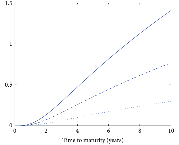
FIGURE 1: The price correction term structure factor \tilde{D} is shown by dotted, dashed, and solid lines as functions of time to maturity, respectively, for (q, s) = (0.2, 0.1) , (0.3, 0.4) , and (0.6, 0.7) .
