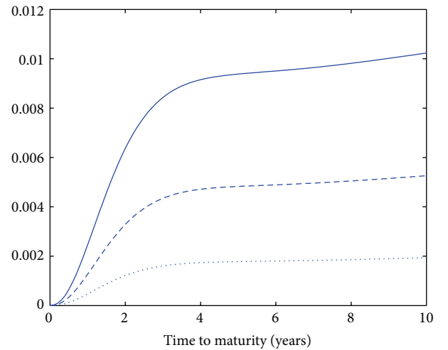
FIGURE 2: The price correction term structure factor \tilde{E} is shown by dotted, dashed and solid lines as functions of time to maturity, respectively, for (u, v) = (0.1, 0.2) , (0.3, 0.5) , and (0.7, 0.8) .
