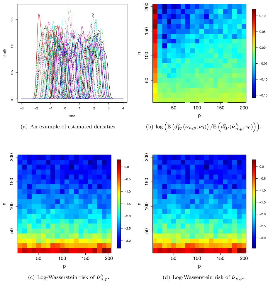
FIG 3. Uniform case - (a) An example of n = 100 densities estimated from data sampled from model (4.1) with the choice of a uniform density f on the interval [0, 1] and n = p = 100 , (b) Logarithm of the ratio \mathbb{E}(d_W^2(\hat{\nu}_{n,p}, \nu_0)) / \mathbb{E}[d_W^2(\hat{\nu}_{n,p}^h, \nu_0)] , (c) Wasserstein risk of the smoothed empirical barycenter \hat{\nu}_{n,p}^h with kernel bandwidths chosen by cross-validation, (d) Wasserstein risk of the non-smoothed empirical barycenter \hat{\nu}_{n,p} . The values of n and p vary from 10 to 200 by an increment of 10.
