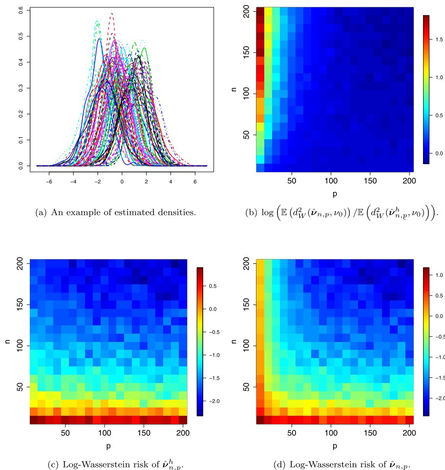
FIG 2. Gaussian case - (a) An example of n = 100 densities estimated from data sampled from model (4.1) with the choice of a standard Gaussian density f truncated to the interval [-3, 3] and n = p = 100 , (b) Logarithm of the ratio \mathbb{E}(d_W^2(\hat{\nu}_{n,p}, \nu_0)) / \mathbb{E}[d_W^2(\hat{\nu}_{n,p}^h, \nu_0)] , (c) Wasserstein risk of the smoothed empirical barycenter \hat{\nu}_{n,p}^h with kernel bandwidths chosen by cross-validation, (d) Wasserstein risk of the non-smoothed empirical barycenter \hat{\nu}_{n,p} . The values of n and p vary from 10 to 200 by an increment of 10.
