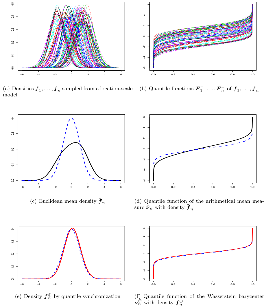
FIG 1. An example of n = 100 random densities (a) with quantile functions (b) sampled from the location-scale model (2.2) with f_0 the standard Gaussian density, \mathbf{a}_i \sim \mathcal{U}([0.8, 1.2]) and \mathbf{b}_i \sim \mathcal{U}([-2, 2]) . (c,d) The solid-black curves are the Euclidean mean \bar{f}_n and its quantile function. (e,f) The solid-red curves are the structural mean f_n^\oplus given by quantile synchronization and the quantile function of the empirical Wasserstein barycenter \nu_n^\oplus . In all the figures, the dashed-blue curves are either the density f_0 or its quantile function in the location-scale model (2.2).
