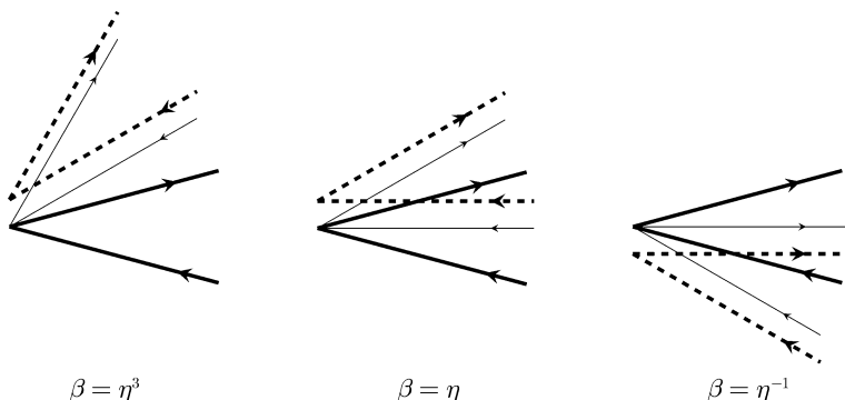
Figure 3.1. W(\pi/m) , f(W(\pi/m)) and \tilde{f}(W(\pi/m)) .
