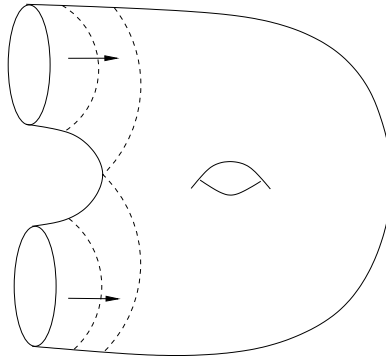
Figure 2: By moving the boundaries of the surface inwards, we find a singular surface.
