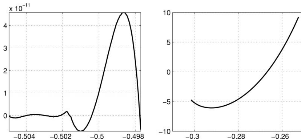
FIGURE 3. The graphs of I(h) on \Gamma_1 and \Gamma_2 .
