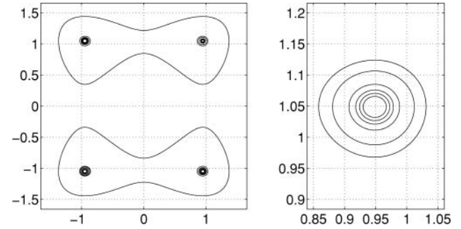
FIGURE 2. The level curves from which the limit cycles bifurcate. On the right is a closeup of \Gamma_1 .
