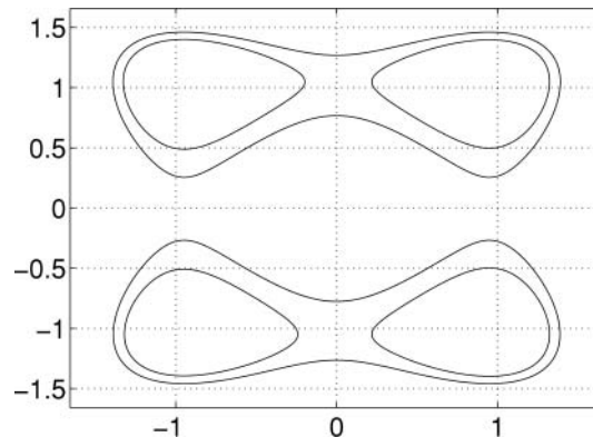
FIGURE 1. The phase portrait of system (2-1).
