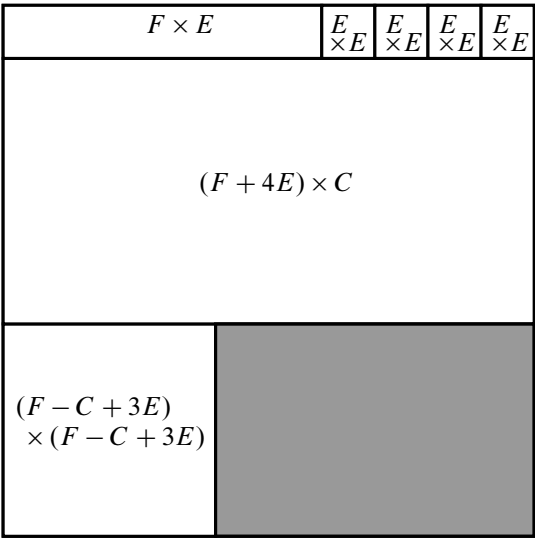
Figure 9: The tiling used to prove Proposition 3.15
